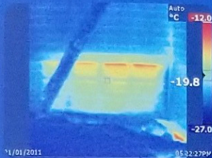
Thermal Image shows heat loss due to lack of insulation
